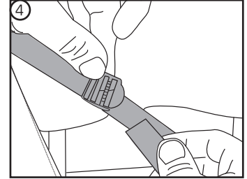
Run the Barrier Extension strap (N) back through its latherlock buckle (P) and pull the strap tight. Repeat steps 3+4 on other side.
