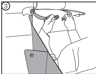
FOR VEHICLES WITHOUT DETACHABLE HEADRESTS: Use the extra strap to attach the Backseat Divider (H) to the back headrest or to the back seat baby hook.
