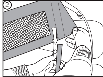
Slide the Barrier Extension (K) on the support columns. Zip the Barrier Extension.
